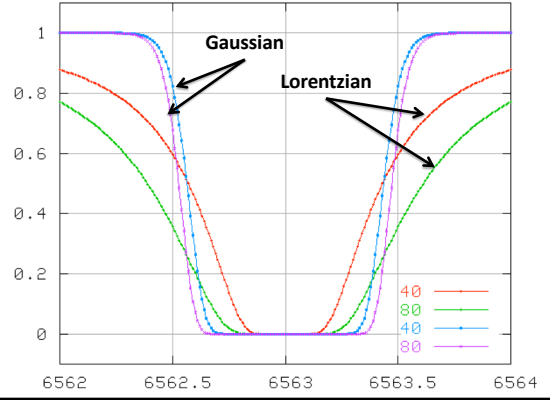
Comparison Gaussian vs. Lorentzian Profiles
