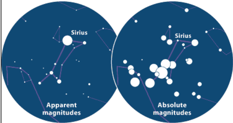
How bright stars appear to us
