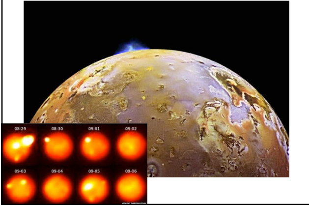
Io Volcanoes
