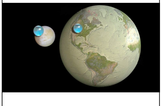
Europa liquid H 2 O vs. Earth
