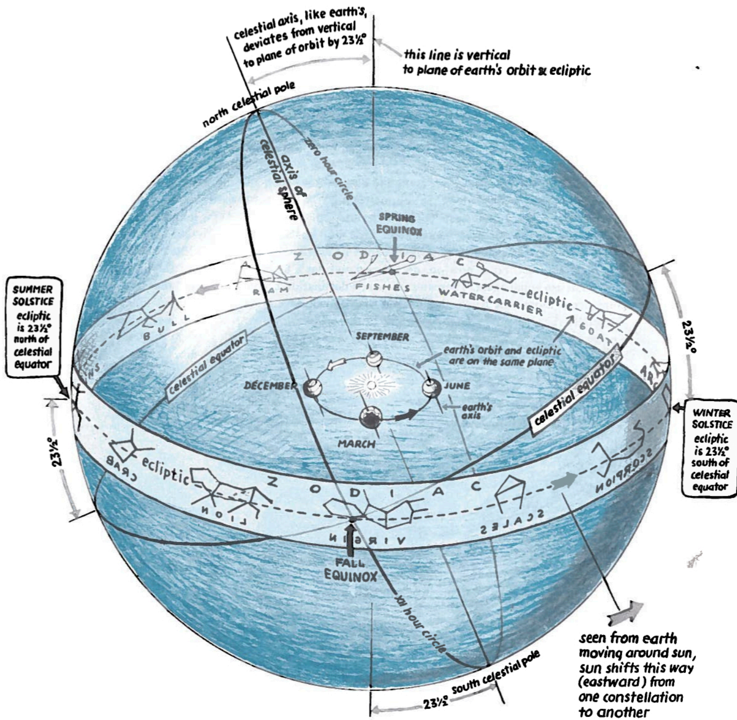
Figure 19: Earth's Orbit inside Celestial Sphere
